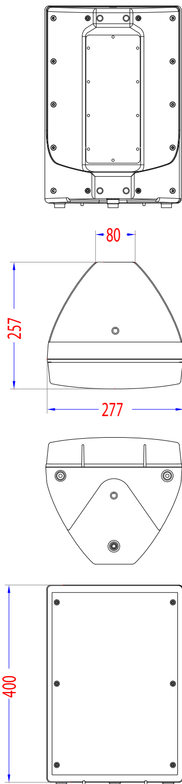
Dimensions (mm)
